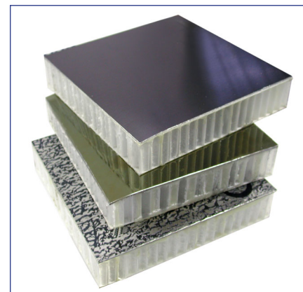
Polypropylene honeycomb
